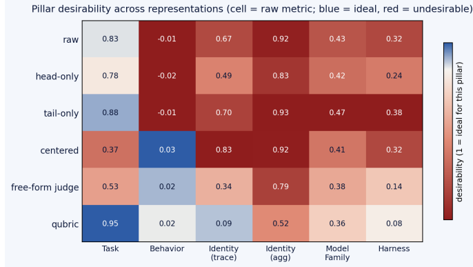
Figure 2: Baselines by pillar: each cell is the raw metric for that axis (columns) under that representation (rows); color is desirability (blue = ideal). Raw-trace variants (head/tail/centered) read authorship; qubric is the only row that is simultaneously task-faithful and authorship-invariant.
