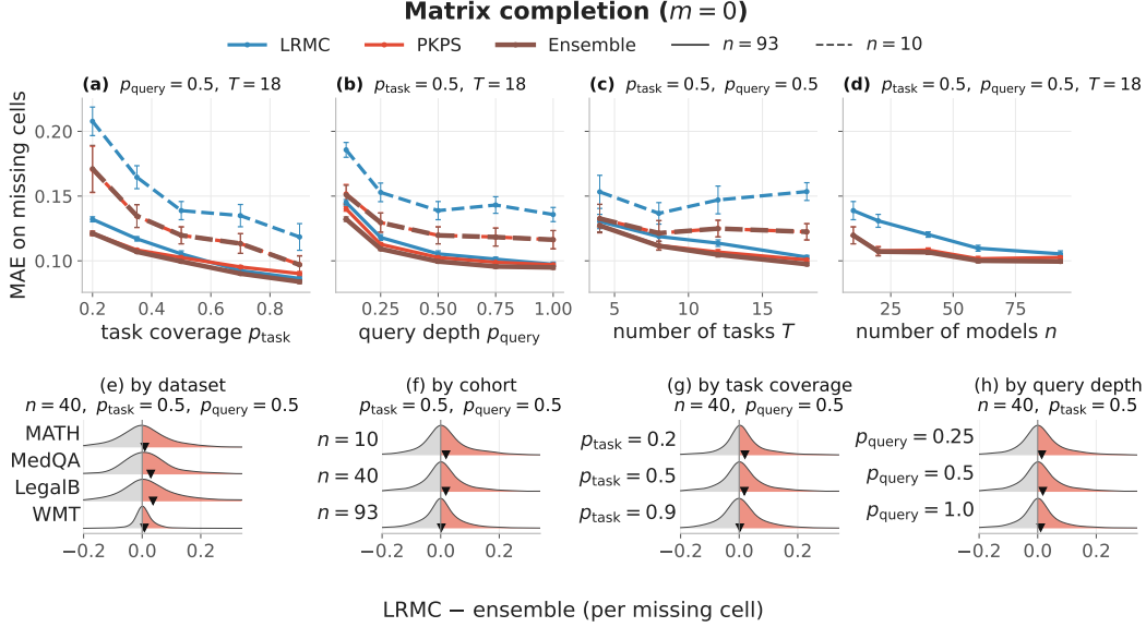
Figure 4: The PKPS embedding rescues the small-cohort regime where LRM collapses for lack of rows, and ties it at full cohort. (a–d) Observe a fraction of (model, task) cells, predict the missing ones (MAE on missing cells, \pm 1 SEM). Colour is method (LRM blue, PKPS red, ensemble brown); line style is cohort (solid n=93 , dashed n=10 ). (e–h) Conditional breakdown: per-missing-cell \Delta = \text{LRM} - \text{ensemble} MAE ( \Delta > 0 , red = win) by dataset, cohort, coverage, and query depth, other levers at their sweep median. Modest and tail-driven on this low-rank suite, but the per-row mean ( \blacktriangledown ) stays positive.
