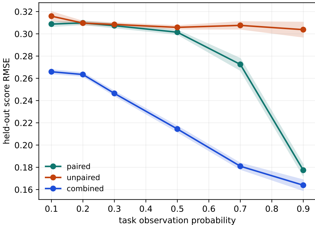
HELM MATH: DoubleKernelDKPS vs task sparsity
