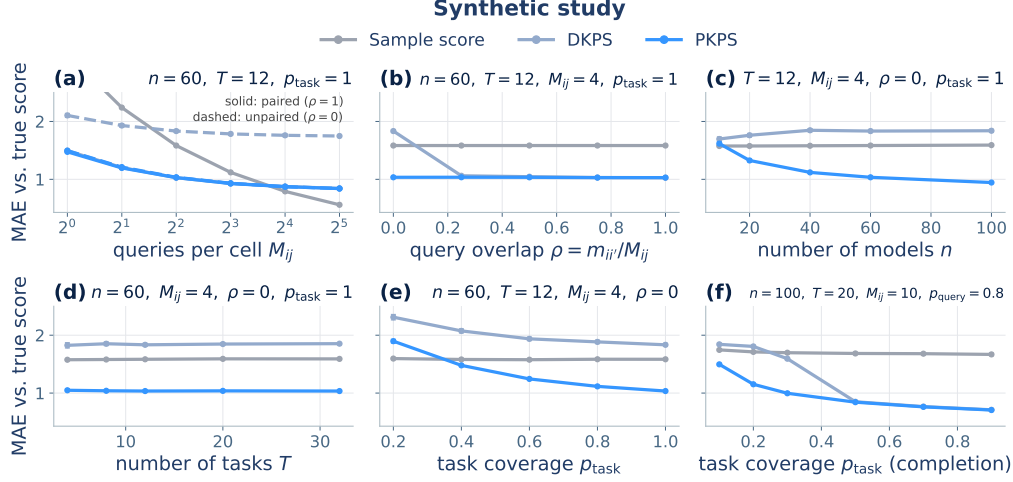
Figure 2: Score MAE on the synthetic benchmark ( \pm 1 SEM over 50 seeds; DKPS light blue, PKPS bright blue, sample score gray; fixed parameters in each panel title). (a–e) Query-efficient evaluation: every observed cell is measured with M_{ij} noisy queries and we predict its true score, as a function of the budget M_{ij} at paired ( \rho=1 , solid) and unpaired ( \rho=0 , dashed) designs (a), the cross-model overlap \rho (b), the cohort size n (c), the number of tasks T (d), and the task coverage p_{\text{task}} (e). (f) Score completion of held-out cells as a function of task coverage; the gray line is the task mean of observed scores (no sample score exists for a held-out cell).
