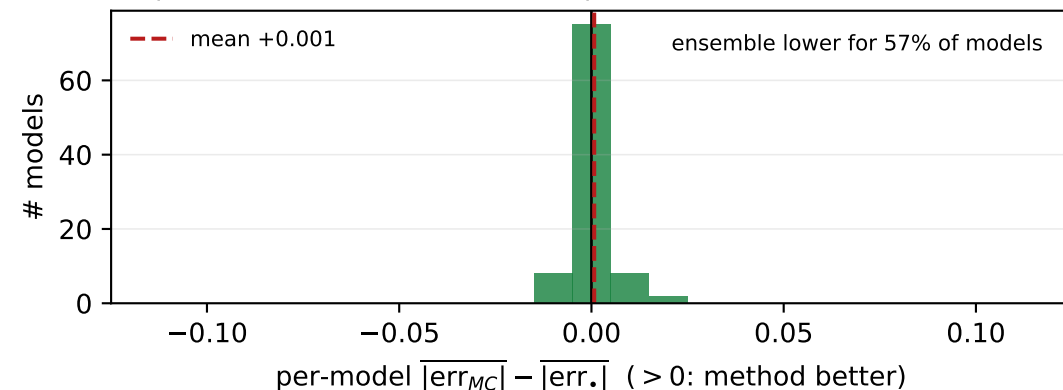
(c) per-model error diff: matrix completion vs ensemble
