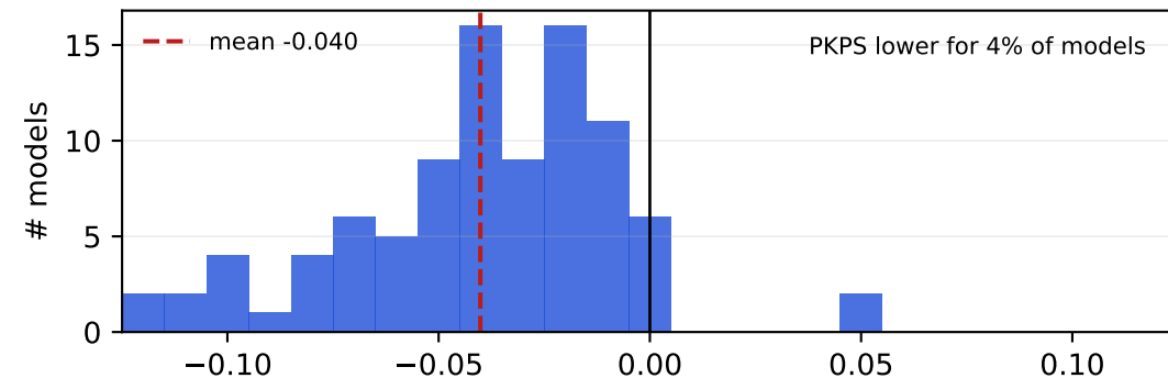
(c) per-model error diff: matrix completion vs ensemble
