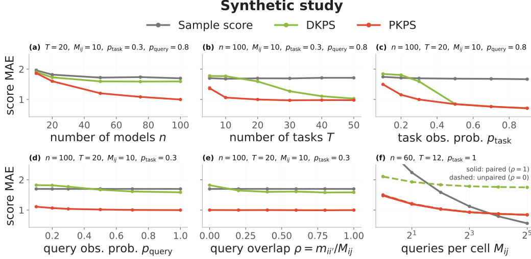
Figure 2: Score MAE on the synthetic benchmark as each lever of the observation process is varied ( \pm 1 SEM over 50 seeds; DKPS green, PKPS red, sample baseline gray; fixed parameters in each panel title). (a–e) Completion of held-out cells as a function of cohort size n , number of tasks T , task coverage p_{\text{task}} , query coverage p_{\text{query}} , and cross-model overlap \rho = m_{ii'}/M_{ij} ; in (e), only DKPS degrades as \rho \rightarrow 0 . (f) Denoising of observed cells: each cell is measured with M_{ij} noisy queries and we predict its true score, at paired ( \rho=1 , solid) and unpaired ( \rho=0 , dashed) designs; PKPS improves on the sample at both, DKPS only when paired.
