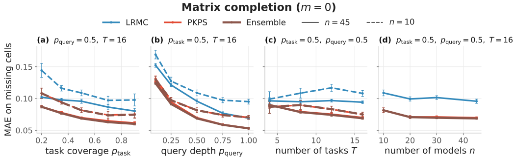
Figure 6: Matrix completion on the Every Eval Ever suite (MAE on missing cells, \pm 1 SEM; solid n=45 , dashed n=10 ). The protocol matches Figure 4. Unlike on the HELM suite, PKPS and the Ensemble outperform LRMC at every operating point, consistent with the higher effective rank of this score matrix.
