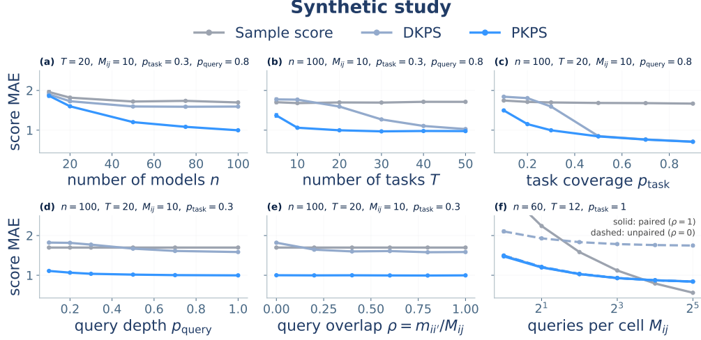
Figure 2: Score MAE on the synthetic benchmark as each lever of the observation process is varied ( \pm 1 SEM over 50 seeds; DKPS light blue, PKPS bright blue, sample score gray; fixed parameters in each panel title). (a–e) Completion of held-out cells as a function of cohort size n , number of tasks T , task coverage p_{\text{task}} , query depth p_{\text{query}} , and cross-model overlap \rho = m_{i'}/M_{ij} ; in (e), only DKPS degrades as \rho \rightarrow 0 . (f) Denoising of observed cells: each cell is measured with M_{ij} noisy queries and we predict its true score, at paired ( \rho=1 , solid) and unpaired ( \rho=0 , dashed) designs; PKPS improves on the sample score at both, DKPS only when paired.
