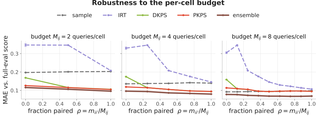
Figure 4: The cliff is robust to the budget. The headline sweep repeated at M_{ij} \in \{2, 4, 8\} queries per cell. At every budget DKPS (green) and IRT (purple) collapse as queries unpair while PKPS (red) holds. MAE vs. full-eval score, \pm 1 SEM.
