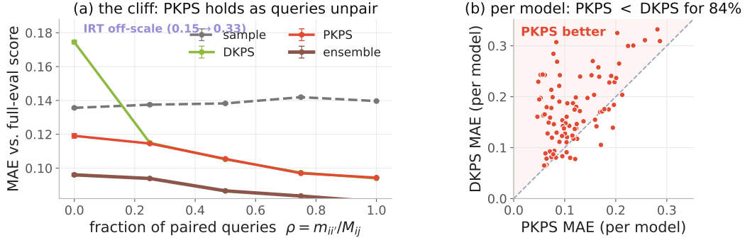
Figure 3: The pairing cliff (headline). Fixed budget M_{ij}=4 queries/cell on the 18-task suite. (a) Sliding from fully paired ( \rho=1 ) to fully unpaired ( \rho=0 ), DKPS (green) collapses—crossing above the raw sample mean (grey)—and IRT runs off-scale (annotated), while PKPS (red) holds and the ensemble (brown) stays lowest. With its bandwidth cross-validated, PKPS coincides with DKPS for \rho \geq 0.25 (CV recovers the delta limit) and pulls ahead as queries unpair. MAE vs. full-eval score, \pm 1 SEM; the y-axis is zoomed to the working band. (b) The same unpaired regime per model: each point is one model’s DKPS vs. PKPS error; PKPS is better for 84% of models (above the diagonal). Only PKPS bridges similar but distinct queries.
