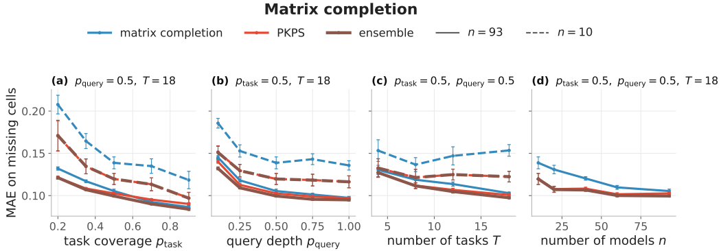
Figure 7: Matrix completion. Observe a fraction of (model, task) cells, predict the missing ones (MAE on missing cells, \pm 1 SEM). Colour is method (low-rank completion blue, PKPS red, ensemble brown); line style is cohort (solid n=93 , dashed n=10 ). The embedding rescues the small-cohort regime where low-rank completion collapses for lack of rows, and ties it at full cohort.
