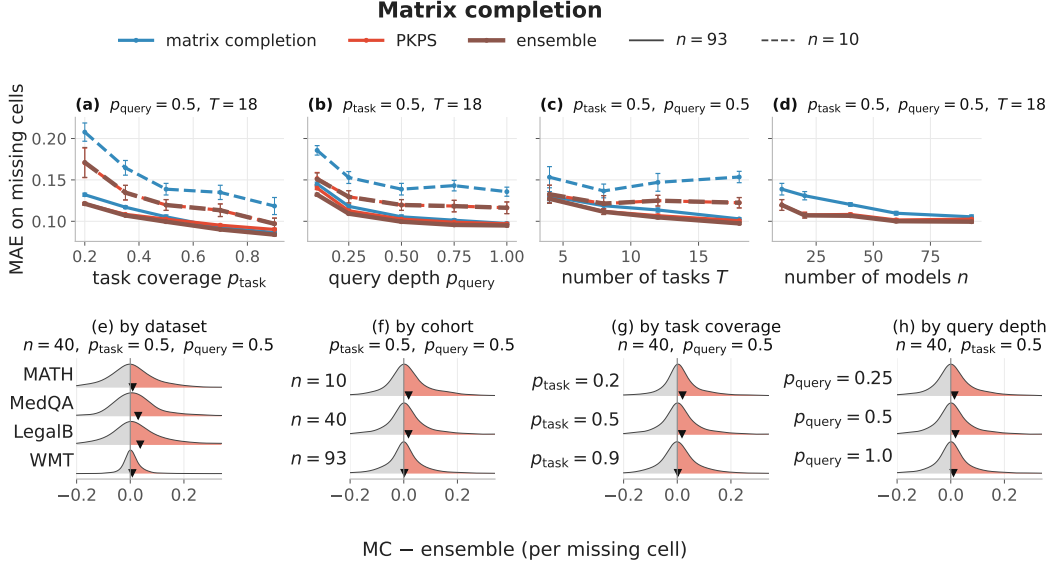
Figure 4: The PKPS embedding rescues the small-cohort regime where low-rank completion collapses for lack of rows, and ties it at full cohort. (a–d) Observe a fraction of (model, task) cells, predict the missing ones (MAE on missing cells, \pm 1 SEM). Colour is method (low-rank completion blue, PKPS red, ensemble brown); line style is cohort (solid n=93 , dashed n=10 ). (e–h) Conditional breakdown: per-missing-cell \Delta = \text{completion} - \text{ensemble} MAE ( \Delta > 0 , red = win) by dataset, cohort, coverage, and query depth, other levers at their sweep median. Modest and tail-driven on this low-rank suite, but the per-row mean ( \blacktriangledown ) stays positive.
