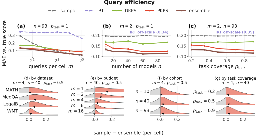
Figure 3: Regression in the PKPS provides query-efficient benchmark prediction relative to the sample score. (a–c) Each model answers m unpaired queries per observed cell; predict its true full-eval score (MAE, \pm 1 SEM). PKPS (red) and the ensemble (brown) denoise far below the raw sample (grey) at small budgets and across cohort (b) and coverage (c); DKPS (green) trails on unpaired queries, and IRT (purple) is poorly identified without a shared item block (omitted from b, c; value annotated). (d–g) Conditional breakdown: per-cell \Delta = \text{sample} - \text{ensemble} MAE ( \Delta > 0 , red = win) by dataset, budget, cohort, and coverage, other levers at their sweep median. Broad but tail-driven; the per-row mean ( \blacktriangledown ) is positive throughout.
