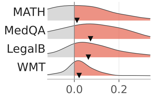
(d) by dataset m = 4, n = 40, p_{\text{task}} = 0.5
