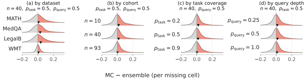
Figure 6: Conditional breakdown of the completion win. Per-missing-cell improvement \Delta = \text{matrix-completion} - \text{ensemble MAE} ( \Delta > 0 , red, the ensemble wins) stacked by dataset, by cohort n , by task coverage p_{\text{task}} , and by query depth p_{\text{query}} , holding the other levers at their sweep median ( n=40, p_{\text{task}}=0.5, p_{\text{query}}=0.5 ). The win is modest and tail-driven on this low-rank suite—the regime most favorable to completion—but the per-row mean ( \blacktriangledown ) stays positive across conditions.
