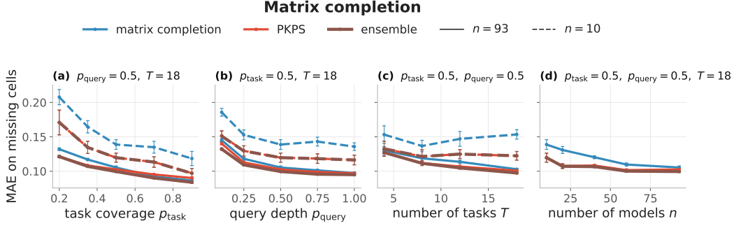
Figure 5: Matrix completion. Observe a fraction of (model, task) cells, predict the missing ones (MAE on missing cells, \pm 1 SEM). Colour is method (low-rank completion blue, PKPS red, ensemble brown); line style is cohort (solid n=93 , dashed n=10 ). The embedding rescues the small-cohort regime where low-rank completion collapses for lack of rows, and ties it at full cohort.
