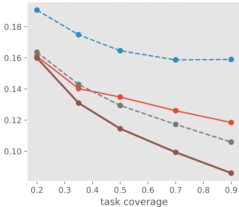
Unified estimation of the full score matrix (MATH): one ensemble beats the best score-only predictor across all three levers
