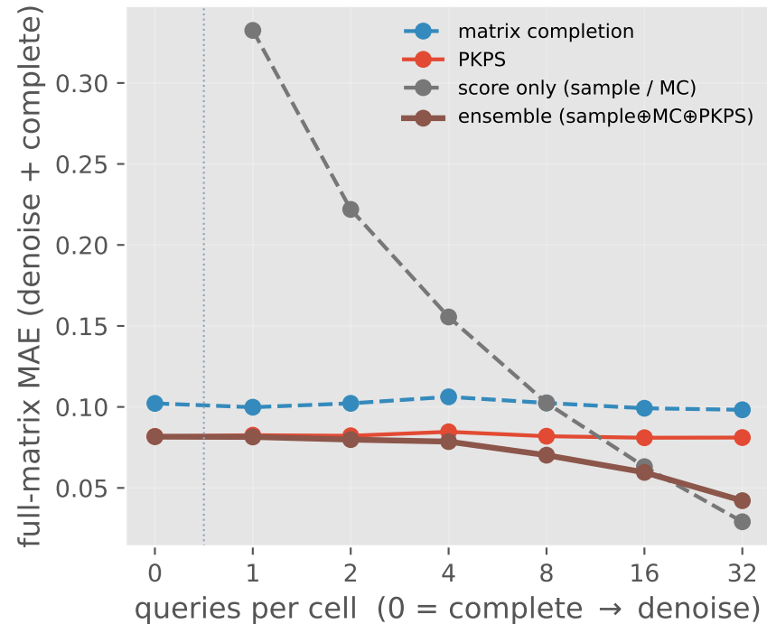
Unified estimation of the full score matrix (MATH): one ensemble beats the best score-only predictor across all three levers
