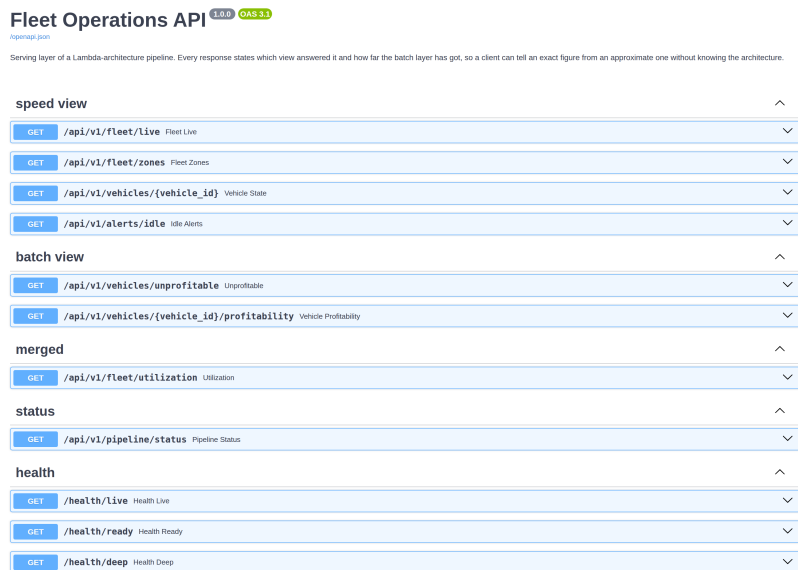
FIGURE 24. The API contract (OpenAPI).
