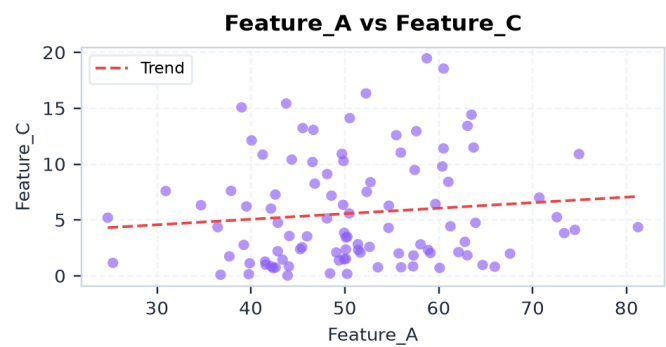
Feature_A vs Feature_C
