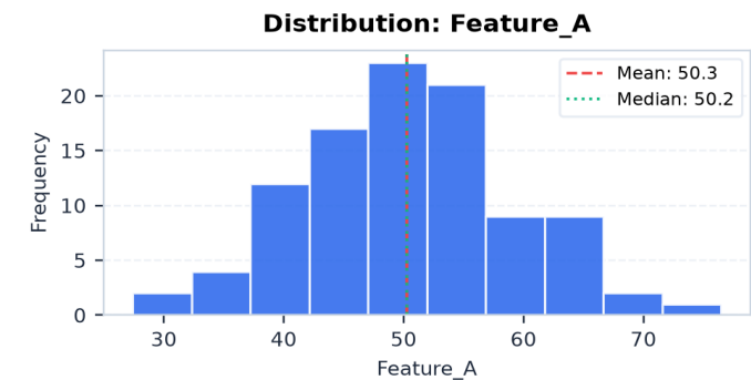
Distribution: Feature_A
