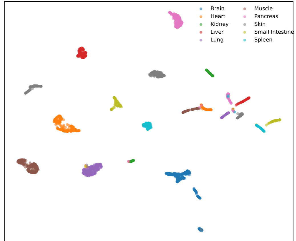
ESPRESSO: tissue
