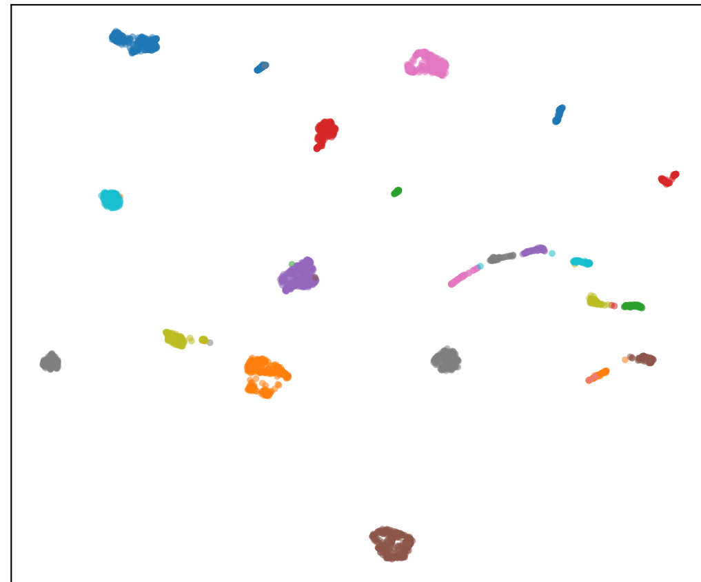
ESPRESSO: tissue
