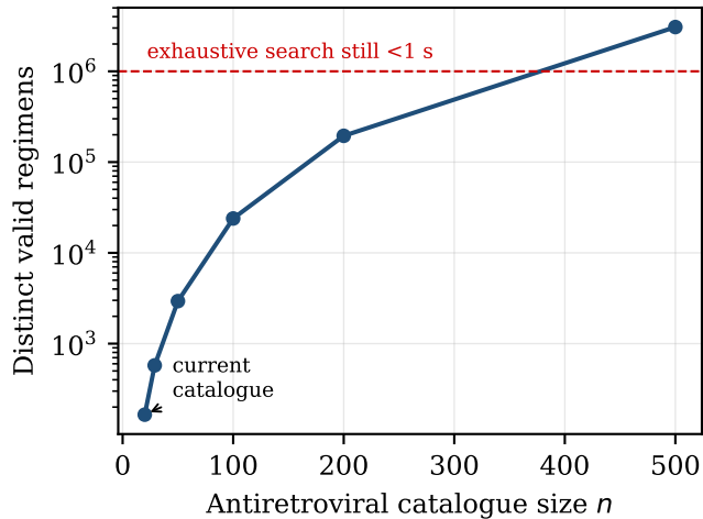
(a) Single-regimen selection: O(n^2m)
