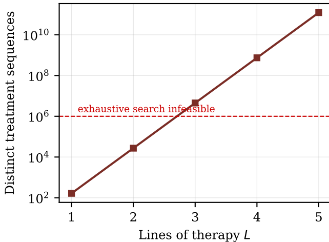
(b) Sequencing: O((n^2m)^L)
