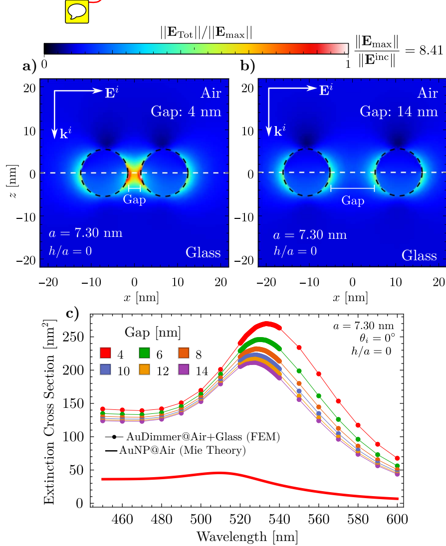
Fig. 2.6: Total electric field spatial distribution \|\mathbf{E}_{\text{Tot}}\| of a AuNP dimer of radius a = 7.30 nm separated by a gap between particles of a) 4 nm and b) 14 nm, illuminated at normal incidence. The AuNP is equally partially embedded in an air matrix and a glass substrate ( h/a = 0 ). c) Extinction cross section of the equally partially embedded AuNP dimer of radius a = 7.30 nm as function of the incident wavelength; the color of each curve corresponds to different values of the gap between the AuNPs of the dimer. In all cases the electromagnetic plane is polarized along the symmetry axis of the dimer.
