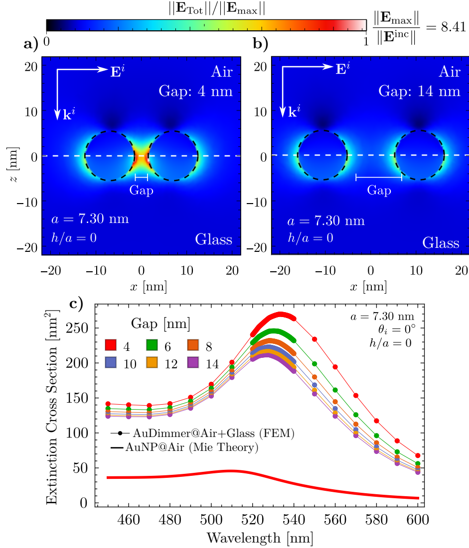
Fig. 2.6: Total electric field spatial distribution ||\mathbf{E}_{\text{Tot}}|| of a AuNP dimmer of radius a = 7.30 nm separated by a gap between particles of a) 4 nm and b) 14 nm, illuminated at normal incidence. The AuNP is equally partially embedded in an air matrix and a glass substrate ( h/a = 0 ). c) Extinction cross section of the equally partially embedded AuNP dimer of radius a = 7.30 nm as function of the incident wavelength; the color of each curve corresponds to different values of the in between the AuNPs of the dimmer. In all cases the electromagnetic plane is polarized along the symmetry axis of the dimmer.
