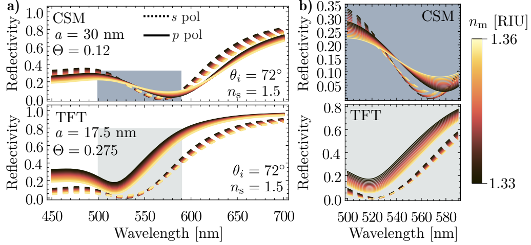
Fig. 3.2: SComparison of reflectivity spectra computed using the Coherent Scattering Model (CSM, upper panels) with a structural scale of a=30\text{nm} , and the Thin Film Theory (TFT, lower panels) with a thickness of a=17.5\text{nm} . In all spectra, solid lines represent pp -polarized light and dashed lines represent ss -polarized light. The curves correspond to varying matrix refractive indices n_m , as indicated by the color legend. (a) Full reflectivity spectra as a function of wavelength. (b) Enlarged view of the shaded regions in (a), highlighting the reflectivity minima and their spectral shift with n_m .
