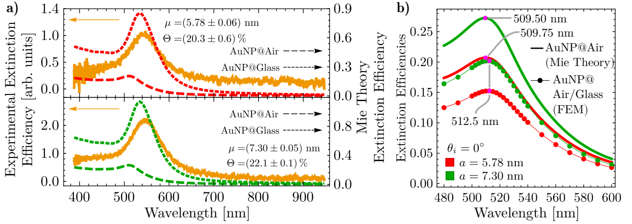
Fig. 2.2: a) Experimental extinction efficiency of the metasurfaces (continuous orange lines) when illuminated at normal incidence, and extinction efficiency of a single AuNP of radius a = 5.78 \text{ nm} (red lines) and a = 7.30 \text{ nm} (green lines) embedded in air (long dashed lines) and in glass (short dashed lines), as given by Mie Theory, as a function of the incident light wavelength. b) Extinction efficiencies as a function of the incidence wavelength, at normal incidence, of a single AuNP embedded in an infinite air matrix (continuous lines) calculated by means of Mie Theory, and in a semiinfinite air matrix supported on a semiinfinite glass substrate (markers) using FEM simulations. The red lines correspond to the calculations of a AuNP with radius a = 5.78 \text{ nm} and the green lines to a = 7.30 \text{ nm} . The magenta markers show the excitation of the LSPR for each case.
