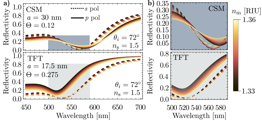
Fig. 3.1: SComparison of reflectivity spectra computed using the Coherent Scattering Model (CSM, upper panels) with a structural scale of a = 30 nm, and the Thin Film Theory (TFT, lower panels) with a thickness of a = 17.5 nm. In all spectra, solid lines represent p polarized light and dashed lines represent s polarized light. The curves correspond to varying matrix refractive indices n_m , as indicated by the color legend. (a) Full reflectivity spectra as a function of wavelength. (b) Enlarged view of the shaded regions in (a), highlighting the reflectivity minima and their spectral shift with n_m .
