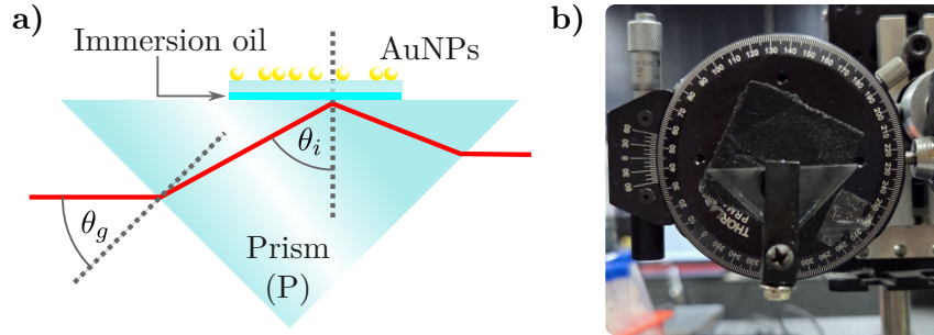
Fig. 1.4: a) Schematic representation of the right-angle prism (P) mounted in the reflectivity measurement setup described in Fig. 1.3 and b) photograph of the prism attached to a goniometer used to control the angle of incidence \theta_i of a light beam on the metasurface of AuNPs (not shown in the photograph). A light beam (red line) entering the prism at an angle \theta_g , measured with the goniometer scale, is refracted inside the prism according to Snell's law. This refraction determines \theta_i at the interface between the prism and the metasurface's substrate, which is optically coupled using an immersion oil layer (cyan line). The dashed gray lines corresponds to the normal direction to any of the planar faces of the prism.
