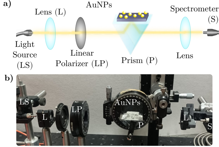
Fig. 1.3: a) Schematic representation and b) photograph of the experimental setup to perform reflectivity spectra measurements. The setup consists in a white light source (LS), whose light beam passes through a lens (L) and linear polarizer (LP) before incising a glass prism (P). The metasurface of AuNPs are coupled with an immersion oil so the AuNPs are illuminated from inside the prism at the desired angle of incidence. The reflected light passes through a second lens (L) into a spectrometer (S).
