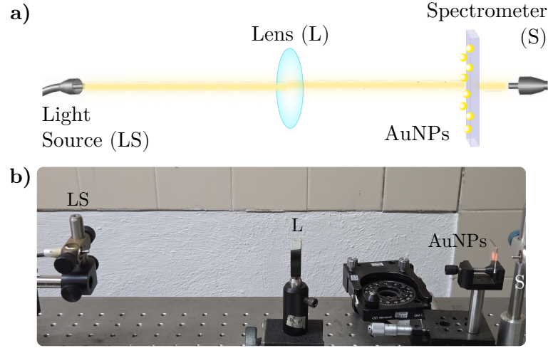
Fig. 1.2: a) Schematic representation and b) photograph of the experimental setup to perform extinction spectra measurements. The setup consists in a white light source (LS), whose light beam is collimated by a lens (L) before illuminating a metasurface of AuNPs at normal incidence. The transmitted light through the metasurface is collected into a spectrometer (S).
