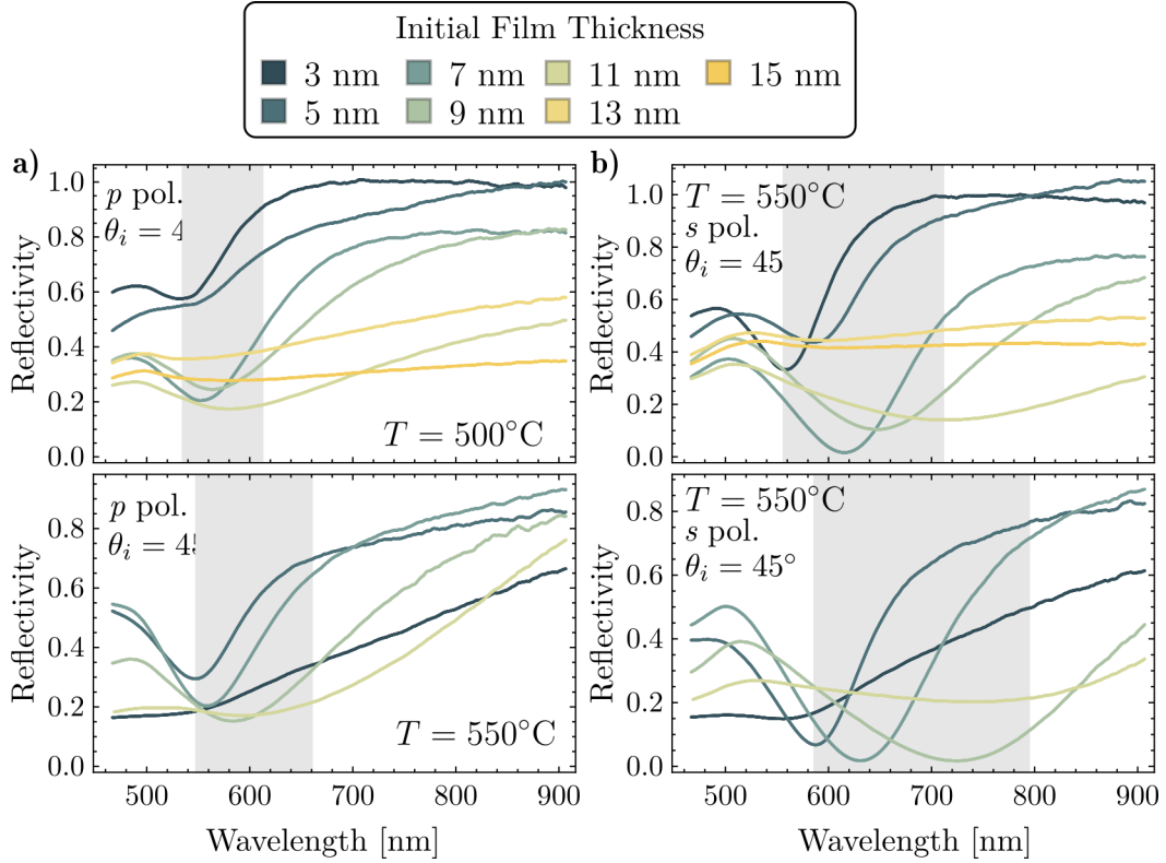
Fig. 2.8: Reflectivity spectra of thermally annealed Au thin films with varying initial thicknesses, measured at an incident angle \theta_i = 45^\circ for (a) p -polarized light at 500^\circ\text{C} (top) and 550^\circ\text{C} (bottom), and (b) s -polarized light at 550^\circ\text{C} . The shaded area marks the spectral region containing the reflectivity minima for most film thicknesses. A clear dependence on thickness, polarization, and annealing temperature is observed, affecting both the position and depth of the plasmonic resonance.
