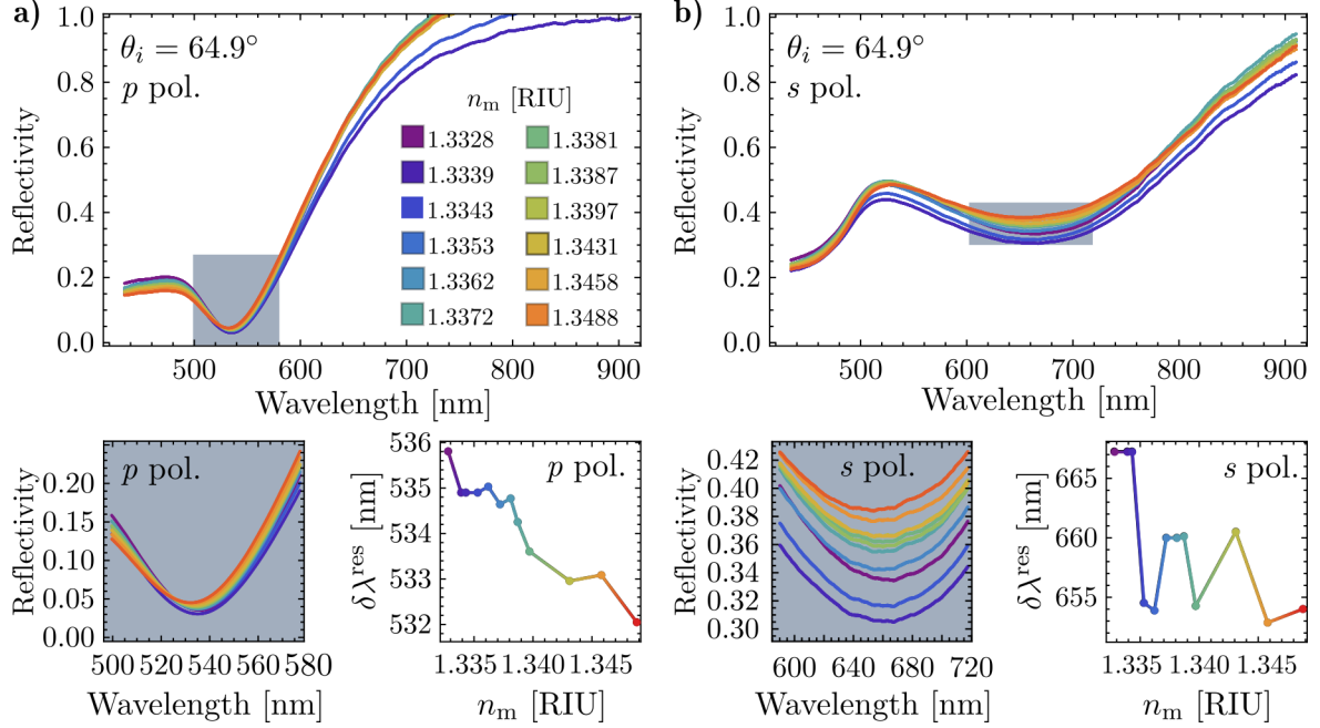
Fig. 3.4: Experimental reflectivity spectra as a function of the incident wavelength for a) p b) s polarized light at an angle of incidence \theta_i = 64.9^\circ of a AuNP metasurface. Each curve in the main frames correspond to measurements with different values of the matrix refractive index n_m . The shaded regions in the main frames highlight spectral windows where the minima of the reflectivity are found and their magnification is shown in the lower left panels for each polarization. The lower right panels show the resonance wavelength shift \delta\lambda^{\text{res}} as a function of n_m .
