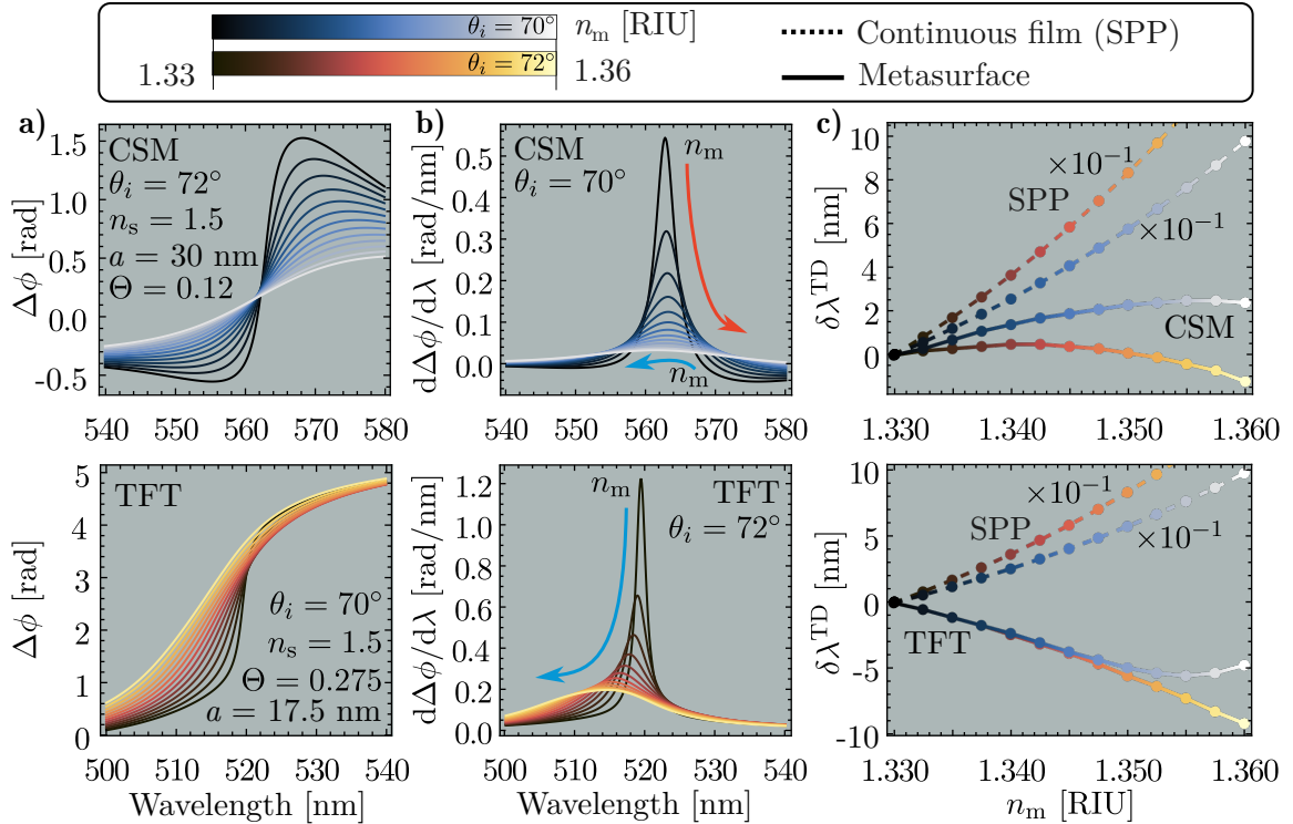
Fig. 3.3: Phase-based sensing scheme with a AuNPs metasurface consisting in the a) phase difference \Delta\phi spectra and b) its spectral derivative d\Delta\phi/d\lambda , both as a function of the incident wavelength for changes in the refractive index n_m of the matrix at an angle of incidence \theta_i of 70^\circ (blue gradient) and 72^\circ (red gradient). The upper panel shows the results with the CSM ( a = 30 nm, \Theta = 0.12 and \theta_i = 70^\circ ) and the lower panel with TFT ( a = 17.5 nm, \Theta = 0.275 and \theta_i = 72^\circ ). The maxima in the d\Delta\phi/d\lambda spectra are located at the TD occurrence wavelength \lambda^{\text{TD}} and their tracking is signaled by the red and blue arrows. c) Spectral shift \delta\lambda^{\text{TD}} as a function of n_m for the proposed metasurfaces (continuous lines) at \theta_i = 70^\circ and \theta_i = 72^\circ ; the spectral shift of the SPP excited in a 50 nm thick continuous gold film (dashed lines) is showed for comparison under an abuse of notation.
