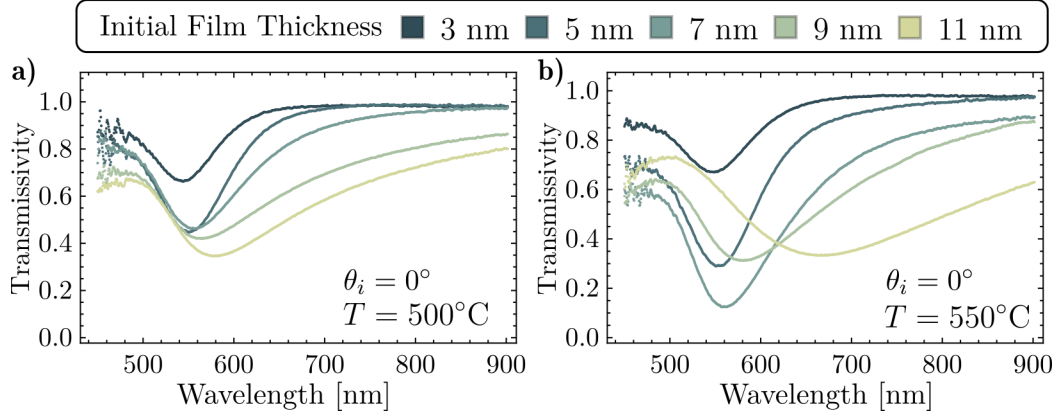
Fig. 2.7: Transmissivity spectra of the synthesized metasurfaces after thermal annealing at a temperature of a) 500^\circ and b) 550^\circ at normal incidence ( \theta_i = 0^\circ ) as function of the incidence wavelength. The color legend on top indicates the nominal thicknesses of the initial deposited gold films prior the dewetting process.
