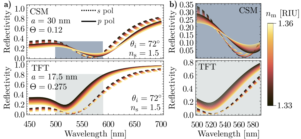
Fig. 3.1: Theoretical reflectivity spectra as function of the incidence wavelength a) in the visible spectra and b) in the spectral window between 500 nm and 590 nm of a metasurface characterized by a mean radius a = 30 nm and surface coverage \Theta = 0.12 (upper panels, calculated with the CSM) and one characterize by a = 17.5 nm and \Theta = 0.275 , (lower panels, calculated with the TFT). A glass substrate with refractive index n_s = 1.5 and an angle of incidence \theta_i = 72^\circ were considered. The continuous (dashed) lines correspond to p ( s ) polarized light and each curves corresponds to varying matrix refractive indices n_m , as indicated by the color legend. The shaded region highlights the window between 500 nm and 590 nm.
