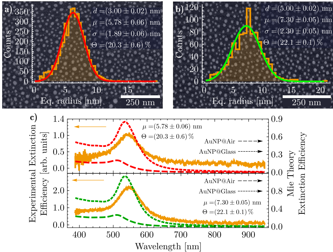
Fig. 2.1: SEM image and histogram of the equivalent radius of the AuNPs in a metasurface fabricated from a gold film with an initial thickness a) d = (3.00 \pm 0.02) \text{ nm} and b) d = (5.00 \pm 0.02) \text{ nm} , both showing a normal distribution of the equivalent radius of the AuNPs with a mean \mu , standard deviation \sigma , and surface coverage \Theta .
