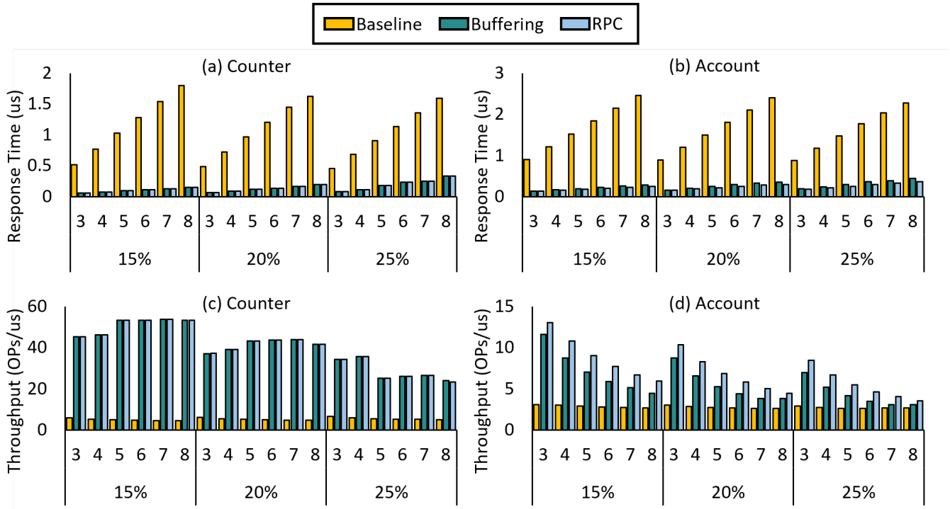
Figure 28: Response time and throughput for one CRDT and one WRDT for three reducible method call implementations.
