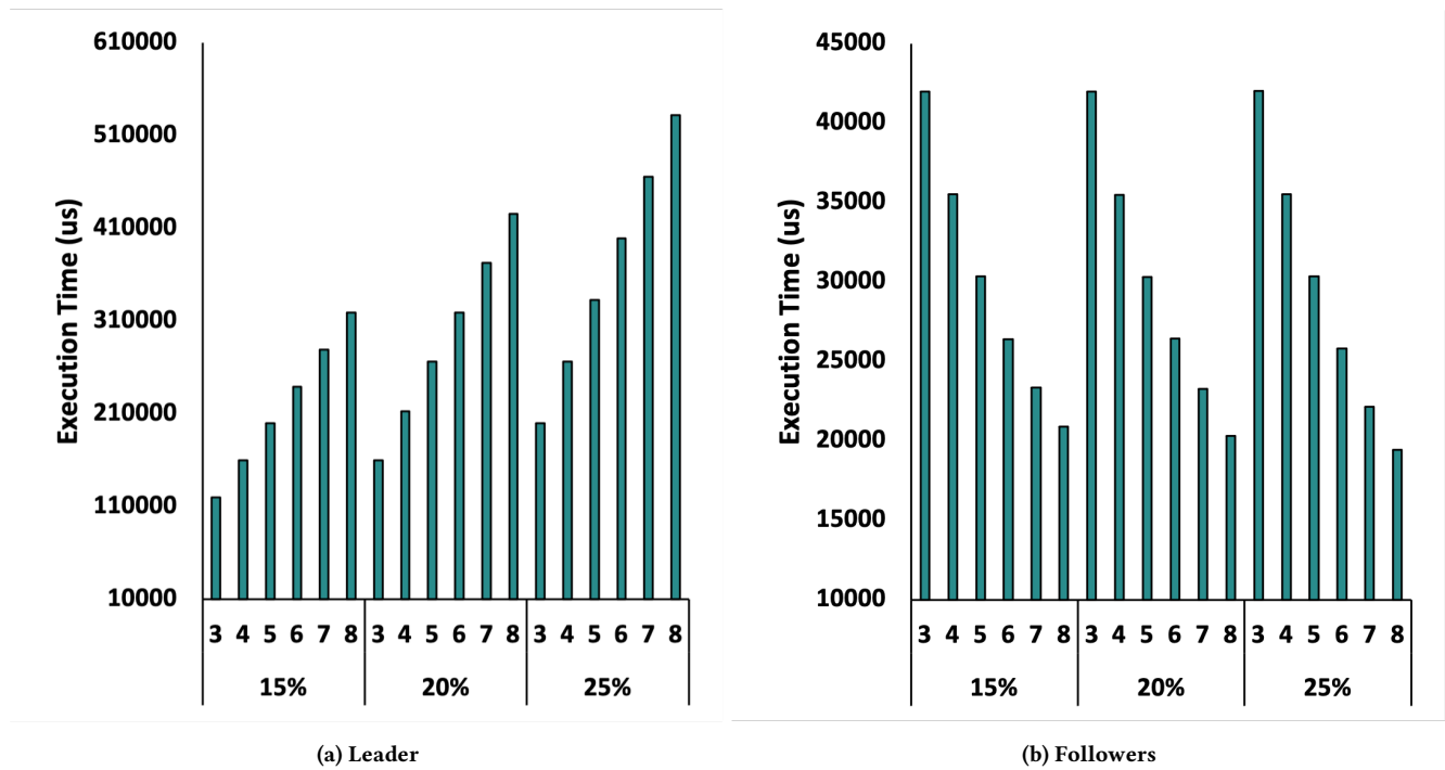
Figure 26: Execution time of leaders and followers in Courseware WRDT
