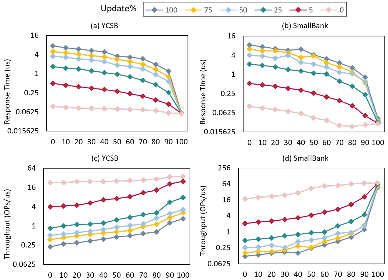
Figure 38: Response time and throughput for YCSB/SmallBank with different percentages of OPs assigned to the FPGA.
