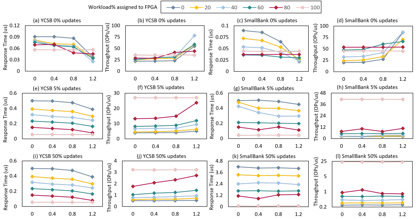
Figure 37: Response time and throughput for YCSB and SmallBank with different \theta values of Zipfian.
