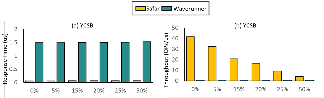
Figure 34: Safar vs. Waverunner response time and throughput on three nodes.
