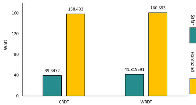
Figure 27: Power Consumption
