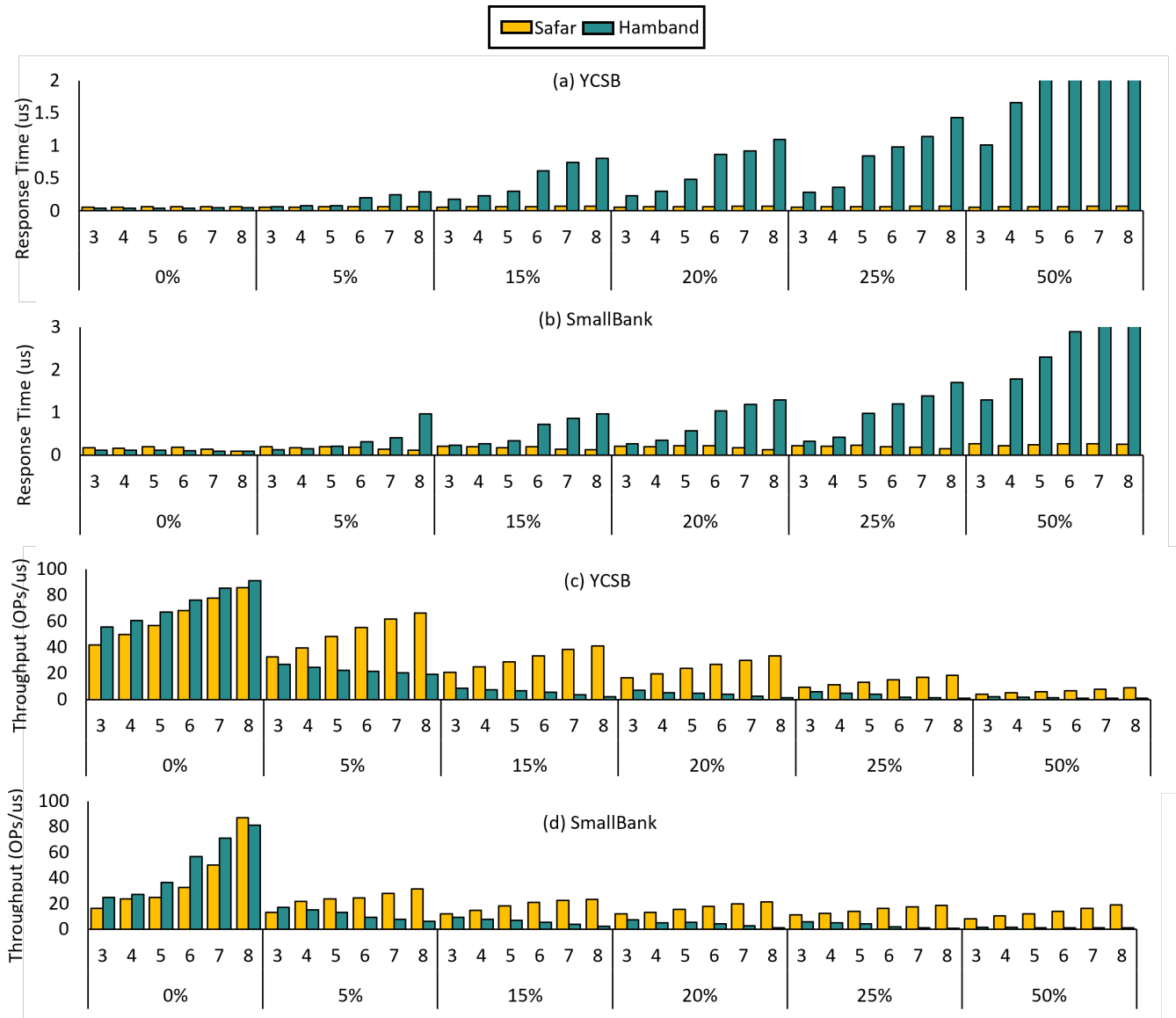
Figure 33: Response time & throughput: YCSB/SmallBank
