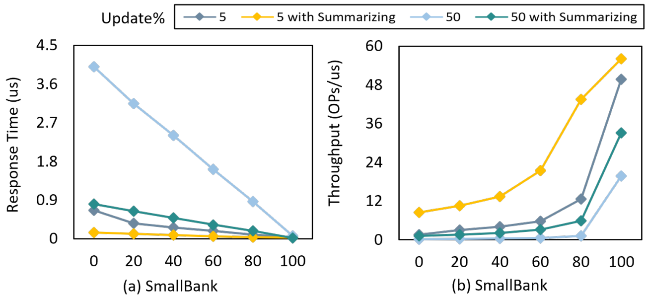
Figure 39: Response time and throughput for SmallBank with a summarization size of 5 in different hybrid percentages.
