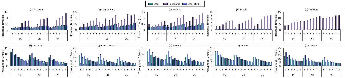
Figure 32: Response Time ( \mu s ) and Throughput (OPs/ \mu s ) of WRDT use-cases
