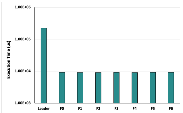
Figure 25: Execution time of all replicas for Bank Account WRDT in a 15% write percentage 8-Node configuration
