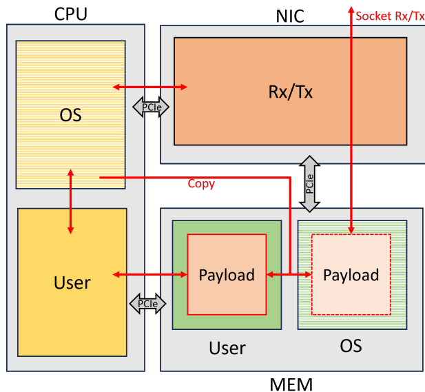
Figure 19: A node in a traditional socket-based network.
