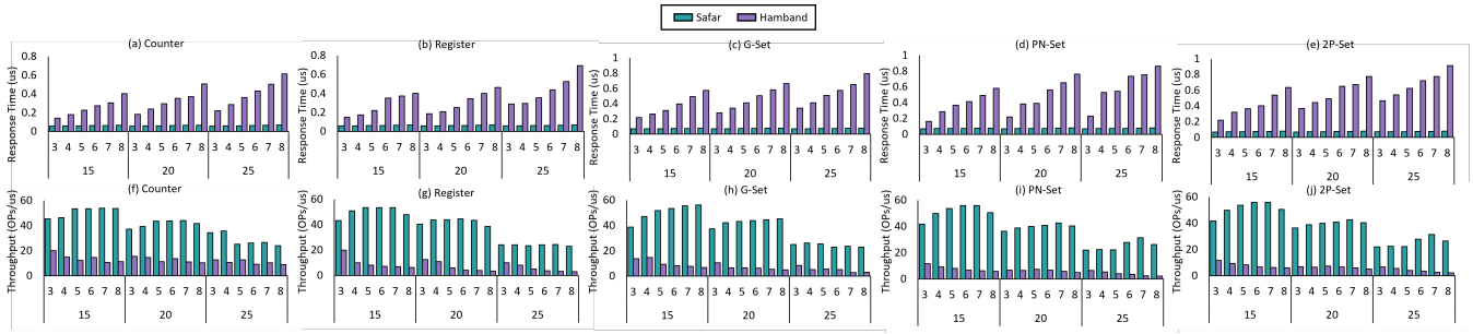
Figure 31: Response Time ( \mu s ) and Throughput (OPs/ \mu s ) of CRDT use-cases
