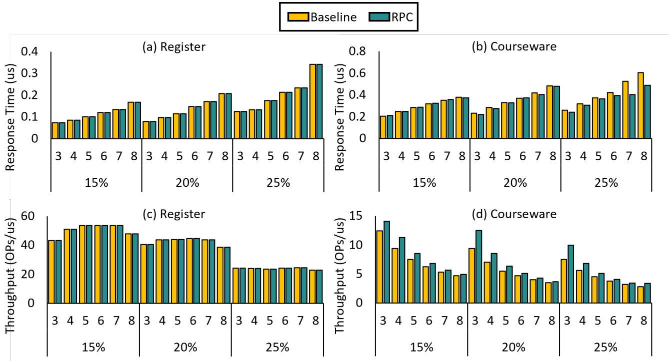
Figure 29: Response time and throughput for one CRDT and one WRDT for two irreducible method call implementations
