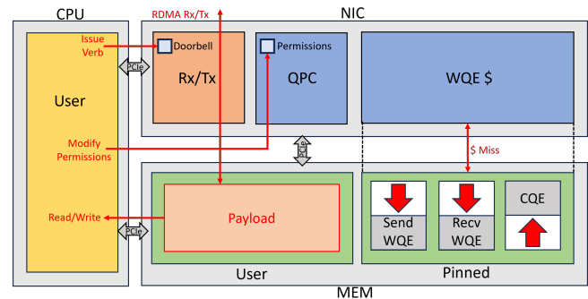
Figure 20: A node in a traditional CPU-based RDMA network.
