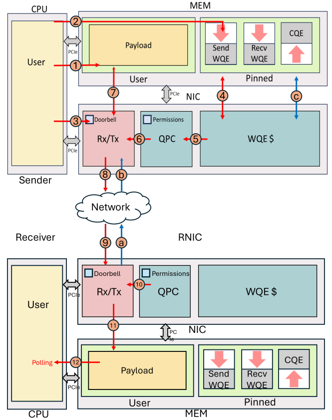
Figure 20: CPU Nic write path
