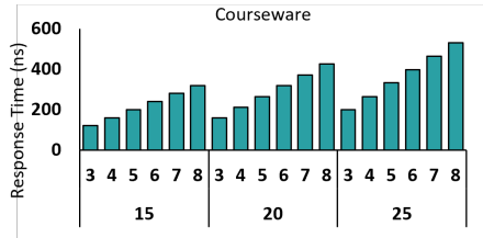
Figure 25: Execution time of leaders in Courseware WRDT
