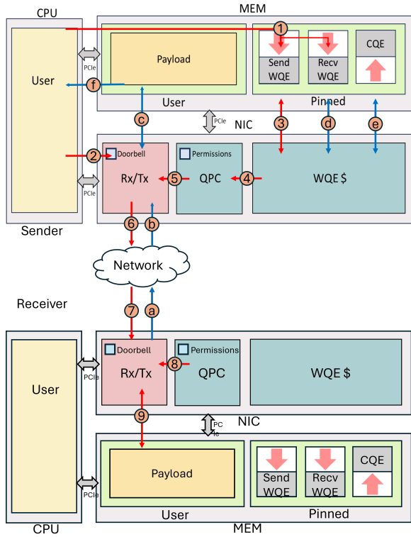
Figure 19: CPU Nic read path
