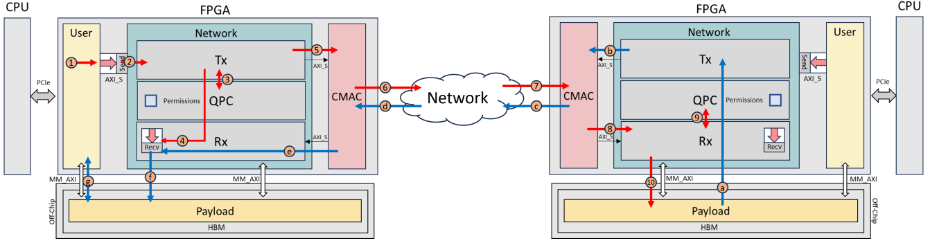
Figure 21: FPGA RDMA read path
