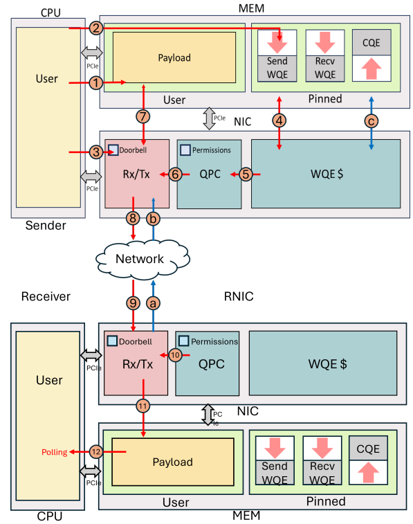
Figure 20: CPU Nic write path
