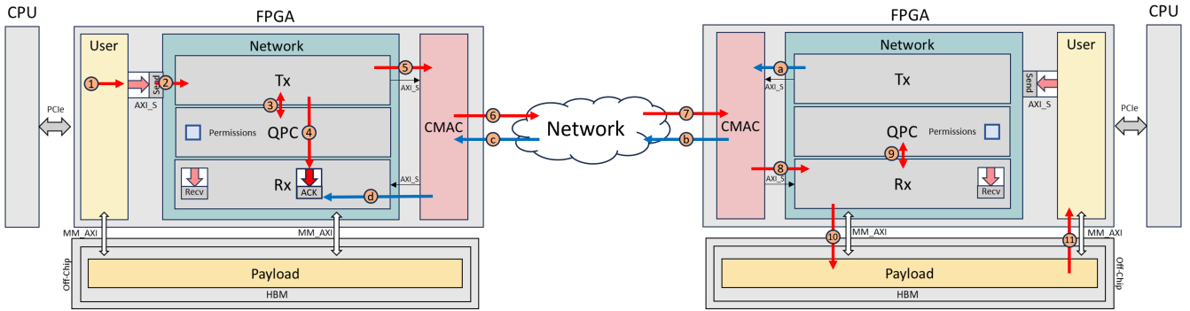
Figure 22: FPGA RDMA write path
