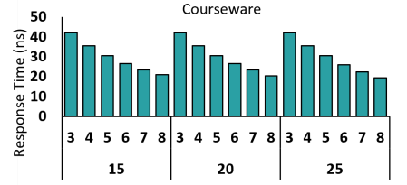
Figure 26: Execution time of followers in Courseware WRDT
