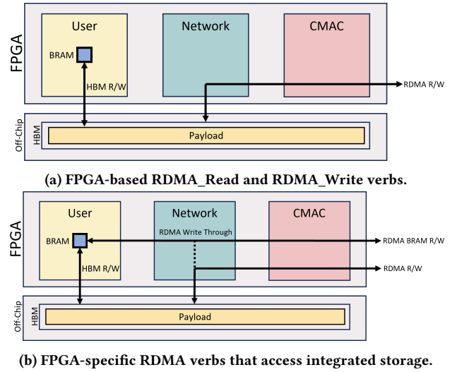
Figure 23: RDMA verbs for network-attached FPGAs.
