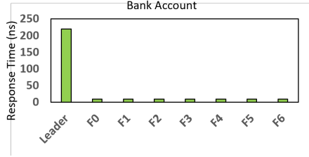
Figure 24: Execution time of all replicas for Bank Account WRDT in a 15% write percentage 8-Node configuration
