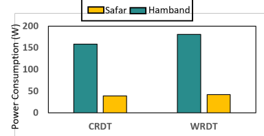
Figure 27: Power Consumption
