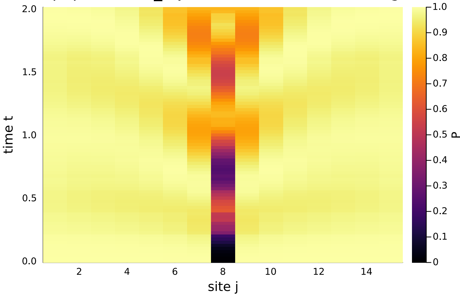
ED population P_0(j,t) ( L=15 , \alpha=0.5 , init=single)
