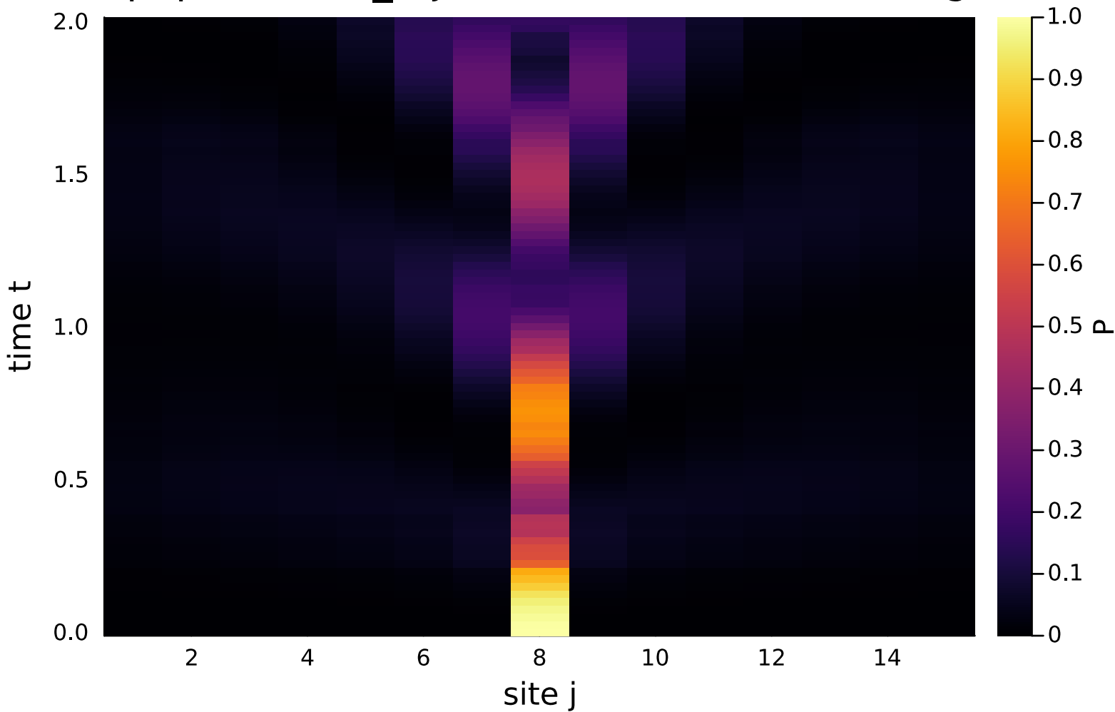
ED population P_1(j,t) ( L=15 , \alpha=0.5 , init=single)
