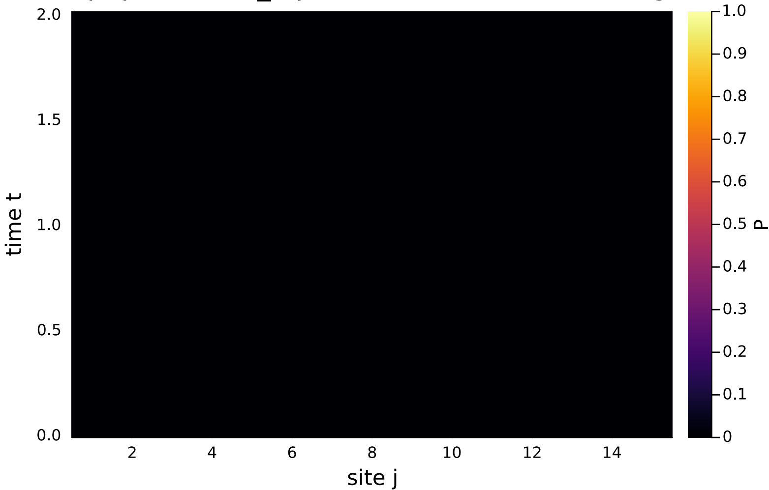
ED population P_2(j,t) ( L=15 , \alpha=0.5 , init=single)
