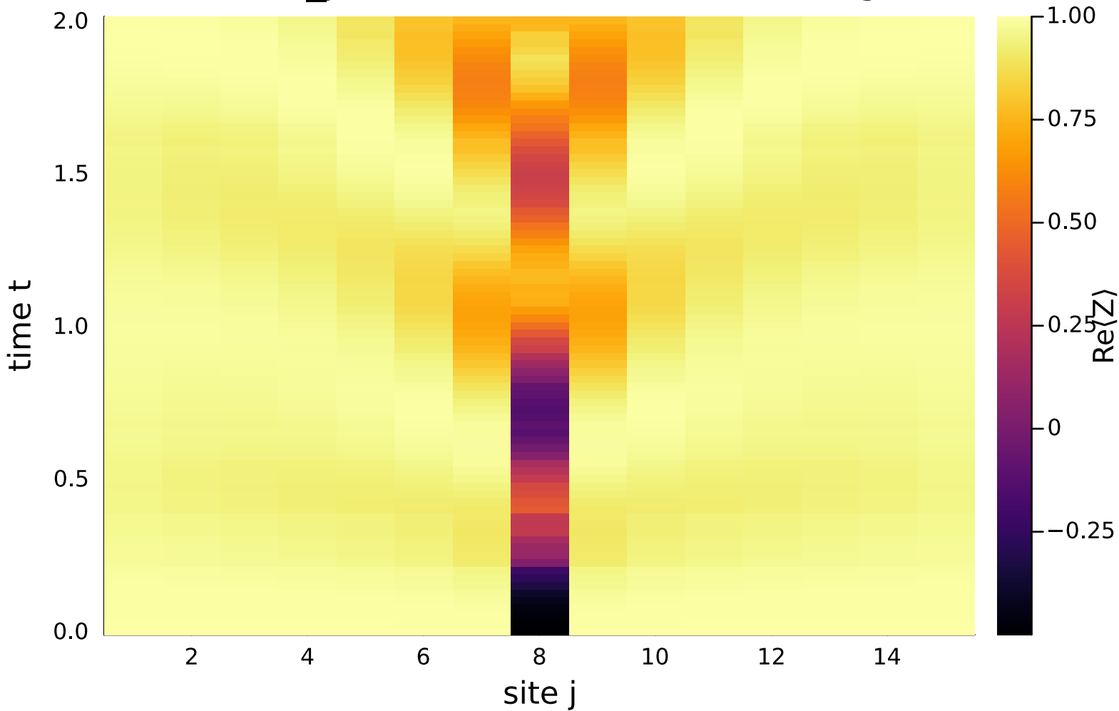
ED \text{Re}\langle Z_j(t) \rangle (L=15, \alpha=0.5 , init=single)
