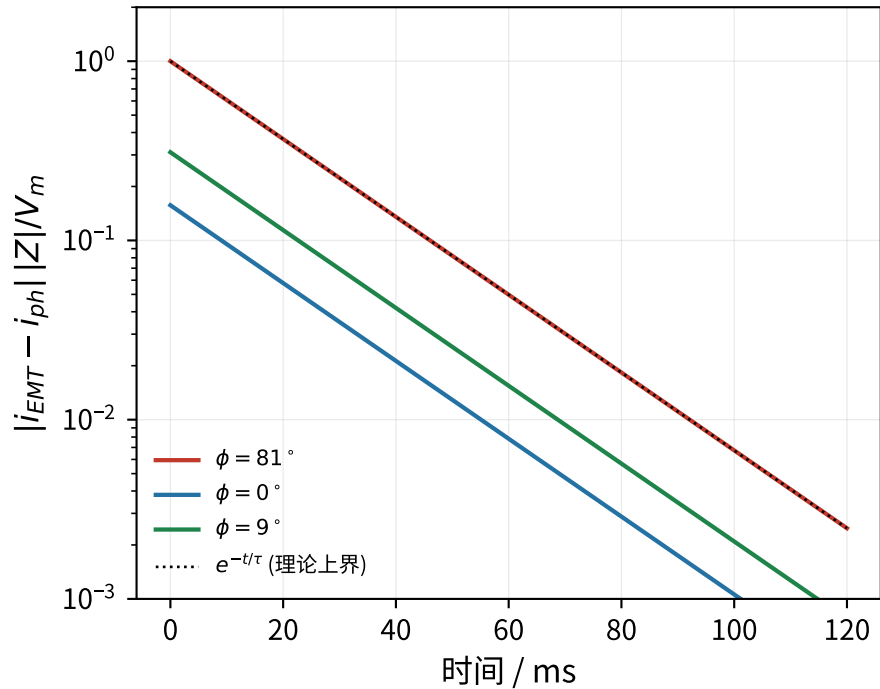
(b) 误差严格按 e^{-t/\tau} 衰减, \tau = L/R
