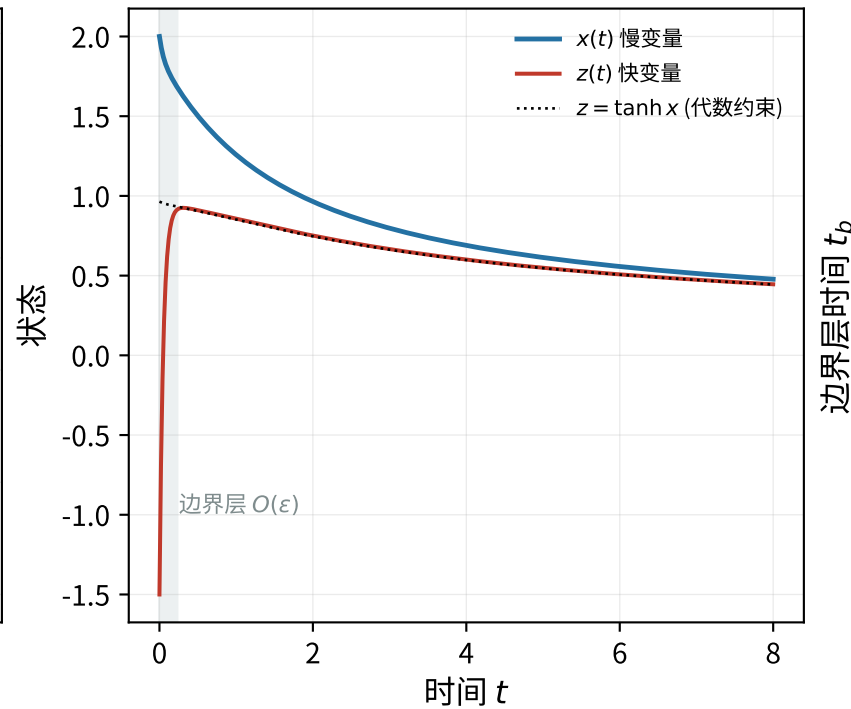
(b) 快动态只在 O(\varepsilon) 边界层内, \varepsilon = 0.05
