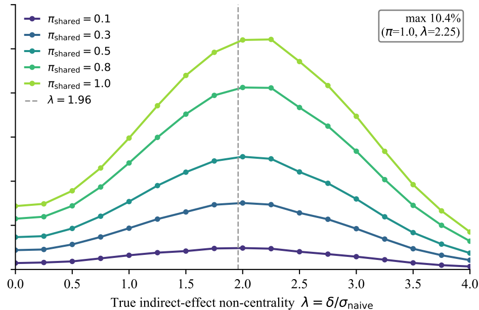
Panel B. Discordant mediation / full overlap ( \rho_{MY} = 1, F = 10 )
