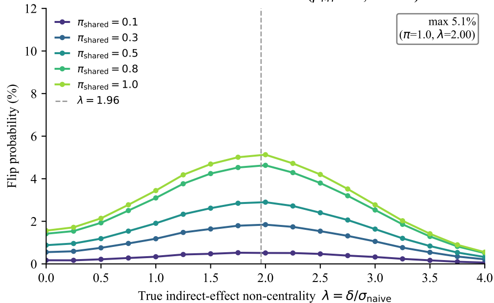
Panel A. Concordant mediation ( \rho_{MY} = 0, F = 10 )
