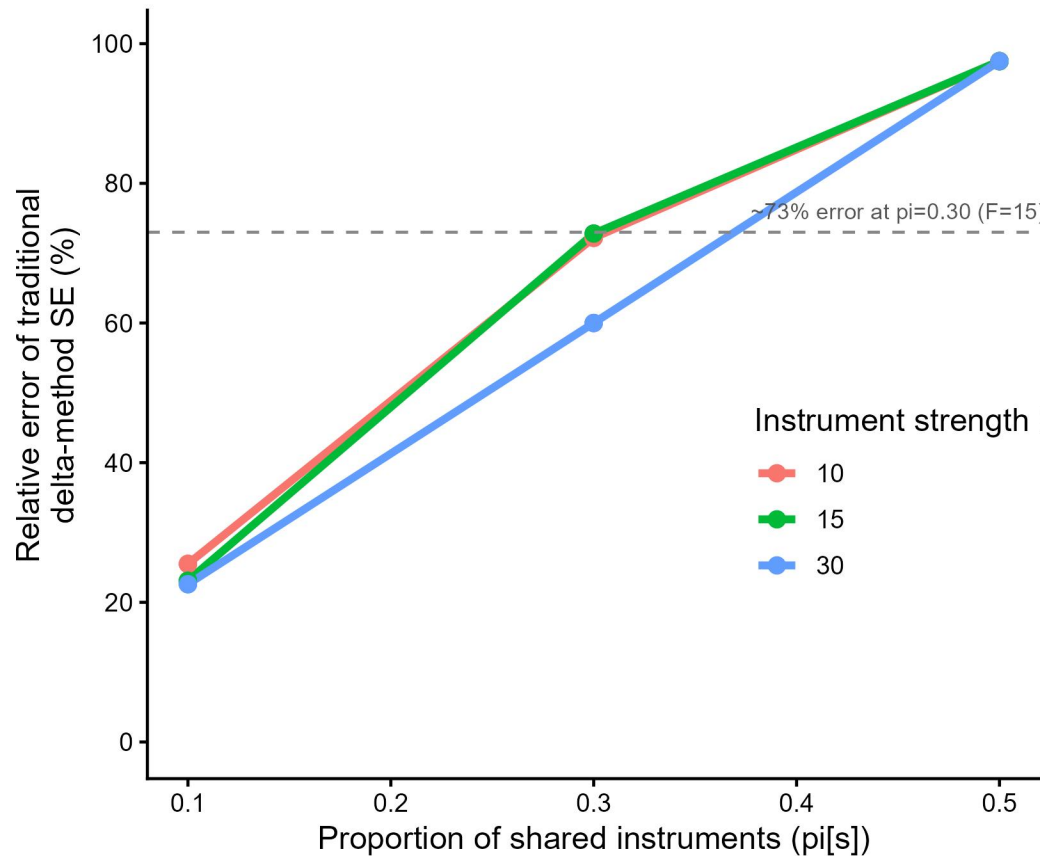
Supplementary Figure S1. Relative error of the traditional delta-method SE and empirical 95% CI coverage from bootstrap validation
