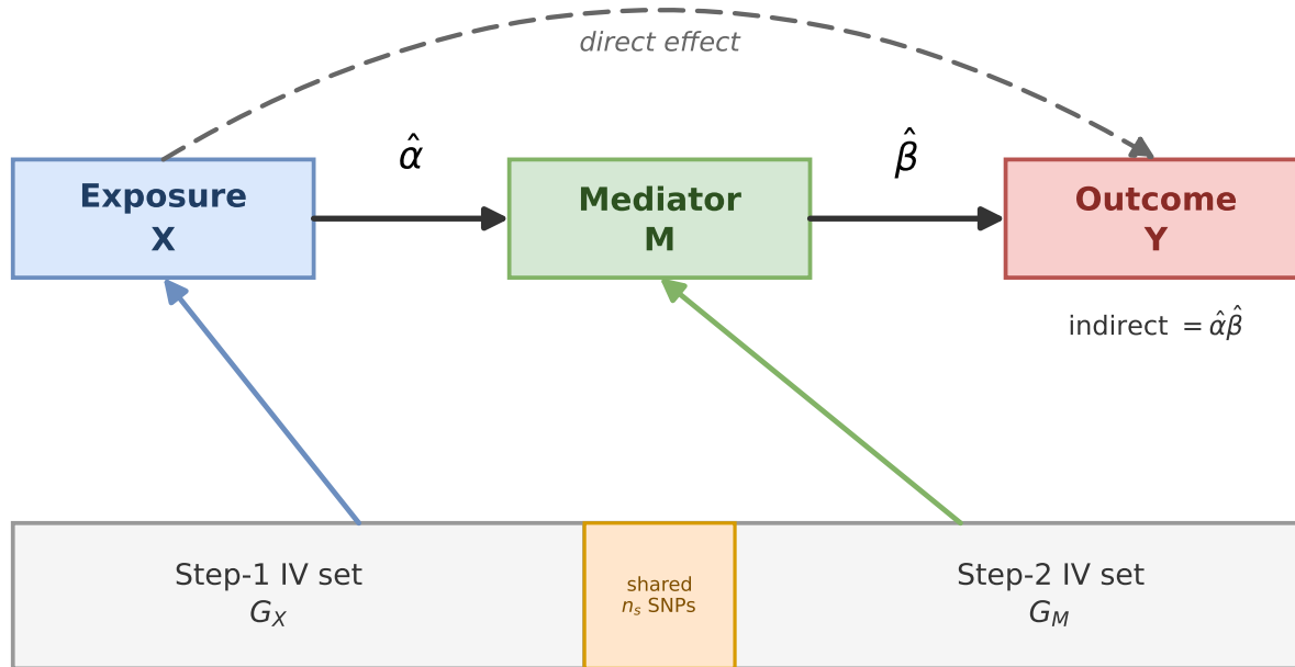
Figure 1. Conceptual diagram of two-step (product-method) MR mediation with overlapping instruments
