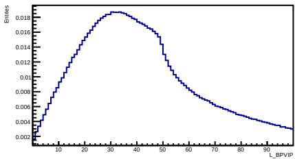
L_BPVIP
