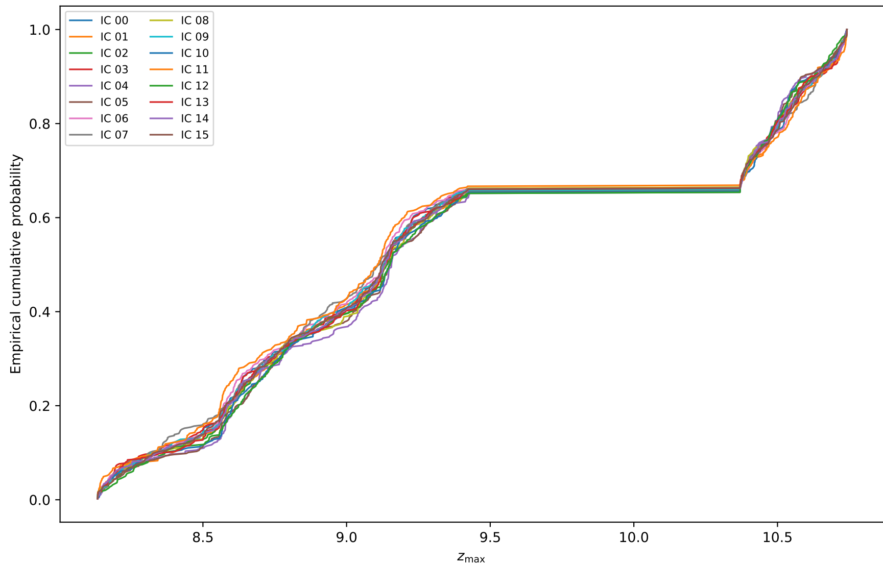
d_1 = 0.38 : distribution of z maxima
