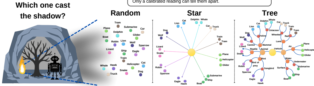
Figure 1: Plato’s cave: a random cloud, a star and a tree cast the same shadow. An observer who sees only shadows cannot tell which object cast them, and a raw \delta is such a shadow: points with no structure, clusters around a center, and a nested hierarchy all read as low \delta . The instrument reads the objects instead of the shadow: the excess separates the random cloud from the other two, and the second test separates the star from the tree.
