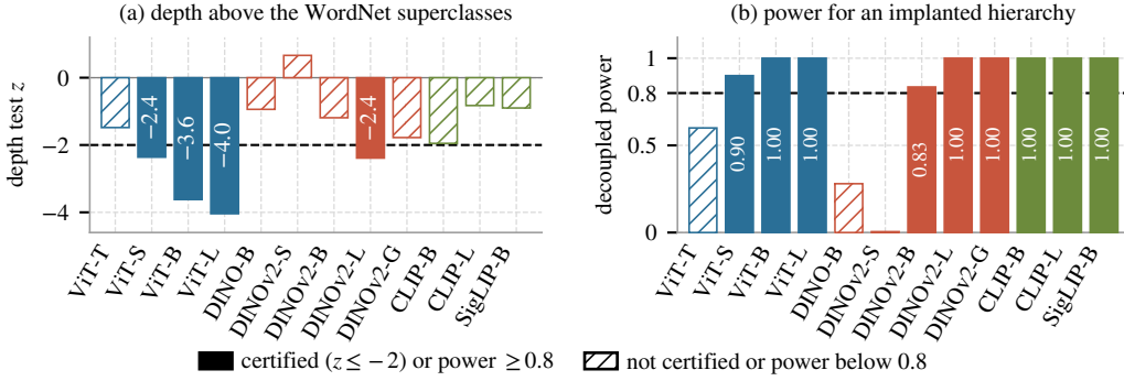
Figure 4: What the depth test certifies, and where it can see a hierarchy. (a) Depth z per backbone, filled when certified; line at z = -2 . (b) Decoupled power for an implanted three-level hierarchy, filled at 0.8 or more; line at 0.8.
