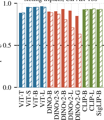
(c) where the tree lives: sibling triplets, CIFAR-100
