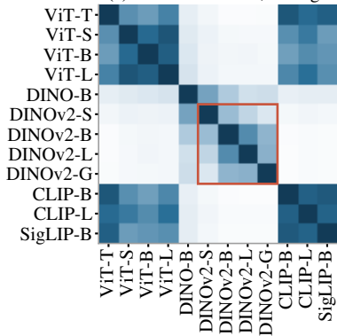
(a) naive: Euclidean, average
