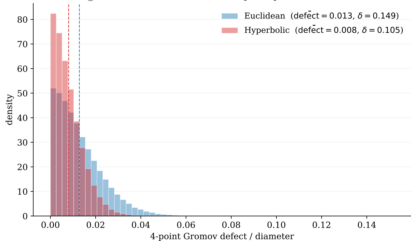
DINOv2_G on CIFAR-100 -- 200K random quadruples of fine-class centroids
