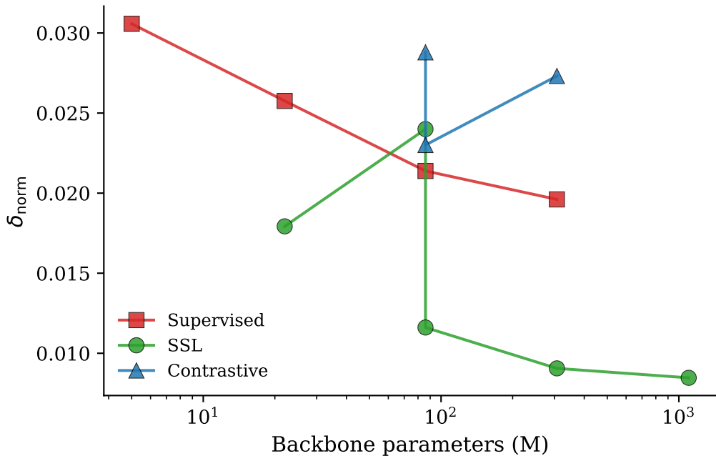
CIFAR-10 -- delta vs. backbone scale
