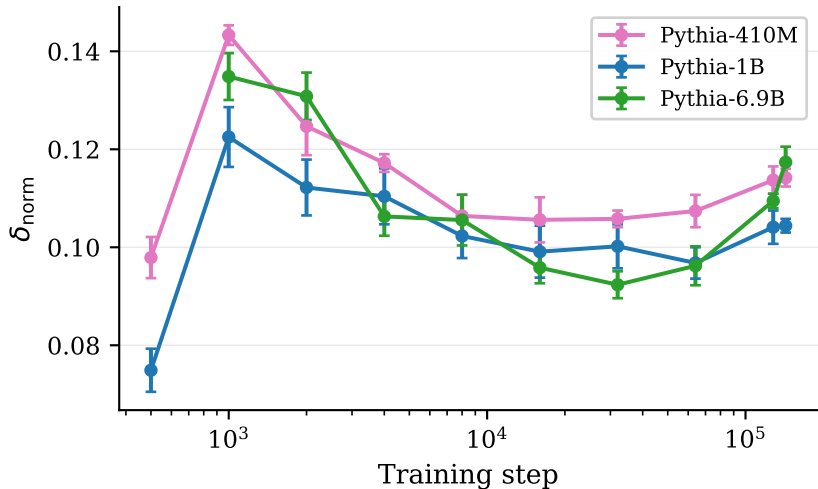
Training dynamics of \delta
