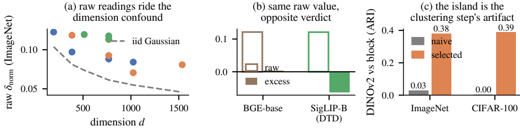
Figure 2: Why calibration: raw \delta cannot be read on its own, and naive tree comparison manufactures islands. (a) Raw \delta_{\text{norm}} rides the dimension confound: iid Gaussians (dashed) drift low as d grows, and the 12 backbones’ ImageNet readings sit on the same slope. (b) A text embedder (BGE-base) and a vision cell (SigLIP-B on DTD) share the same raw value with opposite null verdicts. (c) DINOv2-vs-block tree agreement before and after the configuration control of §5.
