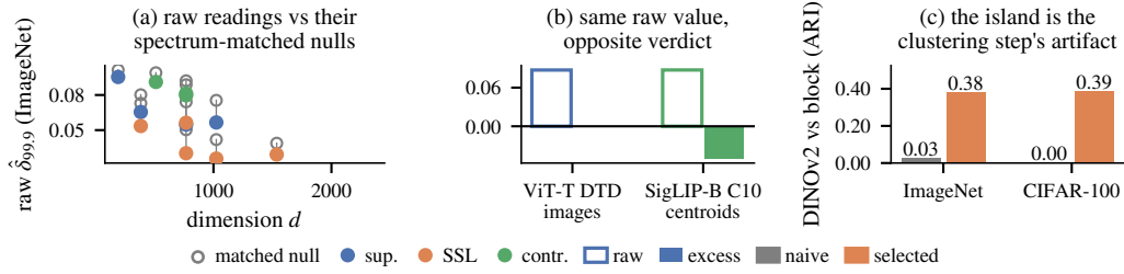
Figure 2: The raw reading cannot be read on its own, and the naive tree comparison manufactures the island. Plotted: (a) the raw reading of the 12 backbones on ImageNet against their matched null means, shown hollow; (b) a sample-level cell (ViT-T on DTD images) and a class-level cell (SigLIP-B on CIFAR-10 centroids) with the same raw reading and opposite verdicts; (c) DINOv2-vs-block tree agreement before and after the configuration control of Section 5.
