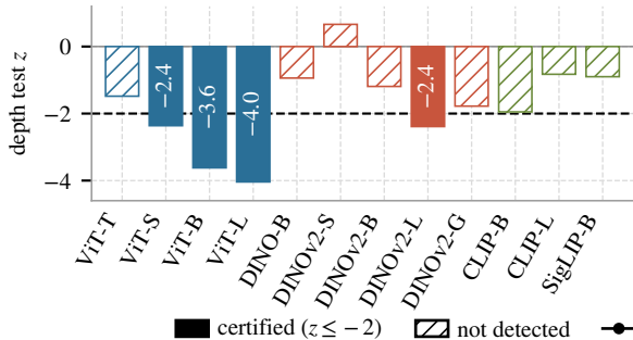
(a) depth above the WordNet superclasses, ImageNet
