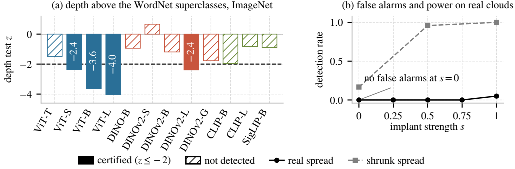
Figure 4: Structure above the superclasses is certified in 4 of 12 ImageNet backbones; it is the alignment of each cluster with its hub, not a hierarchy among the hubs. (a) Depth z per backbone under the matched star, filled and numbered when certified, hatched otherwise, with the certification line at z = -2 . (b) Detection rate against implant strength on the real clouds with the real within-cluster spread (solid) and with it shrunk into the validated range (dashed).
